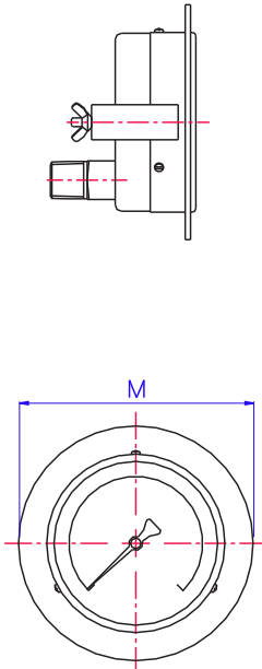
Flush Mounted Clamp Fixing Model - 414
