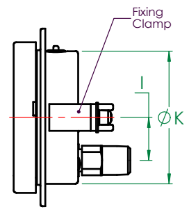
MODEL - 524 Flush Mounted - Clamp Fixing
