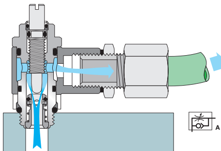
Exhaust Model with External Adjustment
