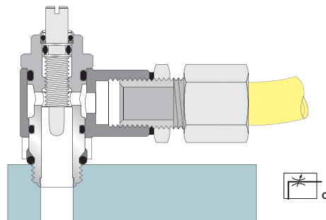
Bi-Directional Model with External Adjustment
